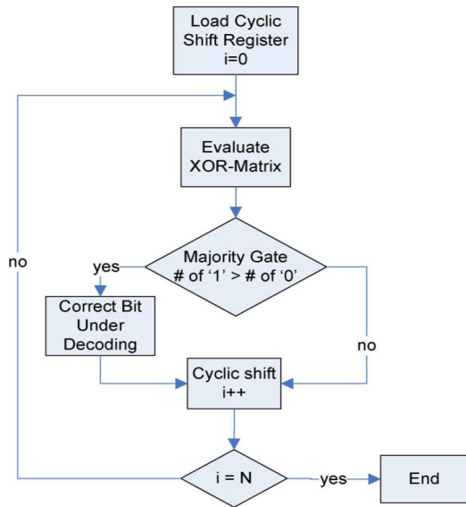
Figure 3. Flowchart of the ML algorithm.
