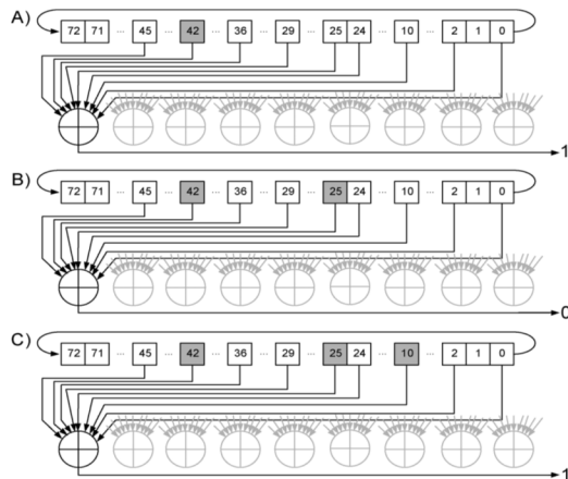
Figure 5. Single check equation of a ML decoder. (a) One bit-flip. (b) Two bit-flips. (c) Three bit-flips.
